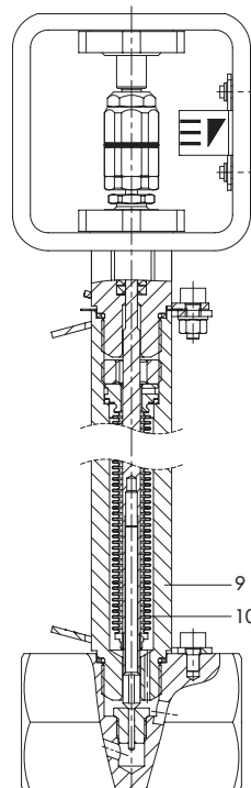
Fig. 5: Type 3510 Valve, globe valve with metal bellows seal
