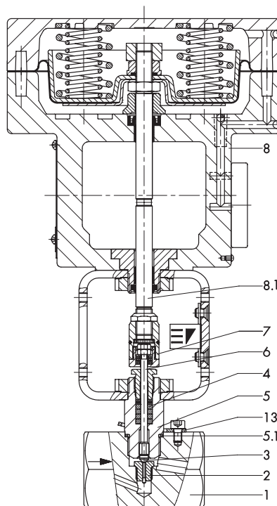
Fig. 4: Type 3510-7 Control Valve
