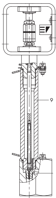
Fig. 3: Type 3510 Valve, angle valve with insulating section
